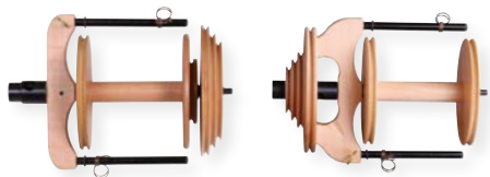
sliding hook flyers
